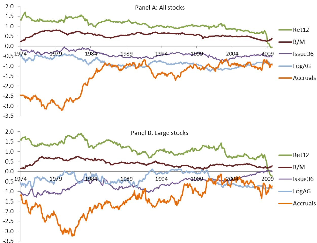
Fig. 1. Ten-year rolling slope estimates, 1974–2009
