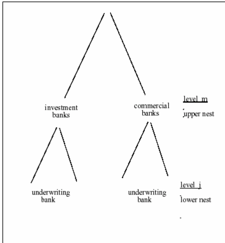
Figure 1. Firm's choice set. This figure specifies the nest structure used in the demand model.
